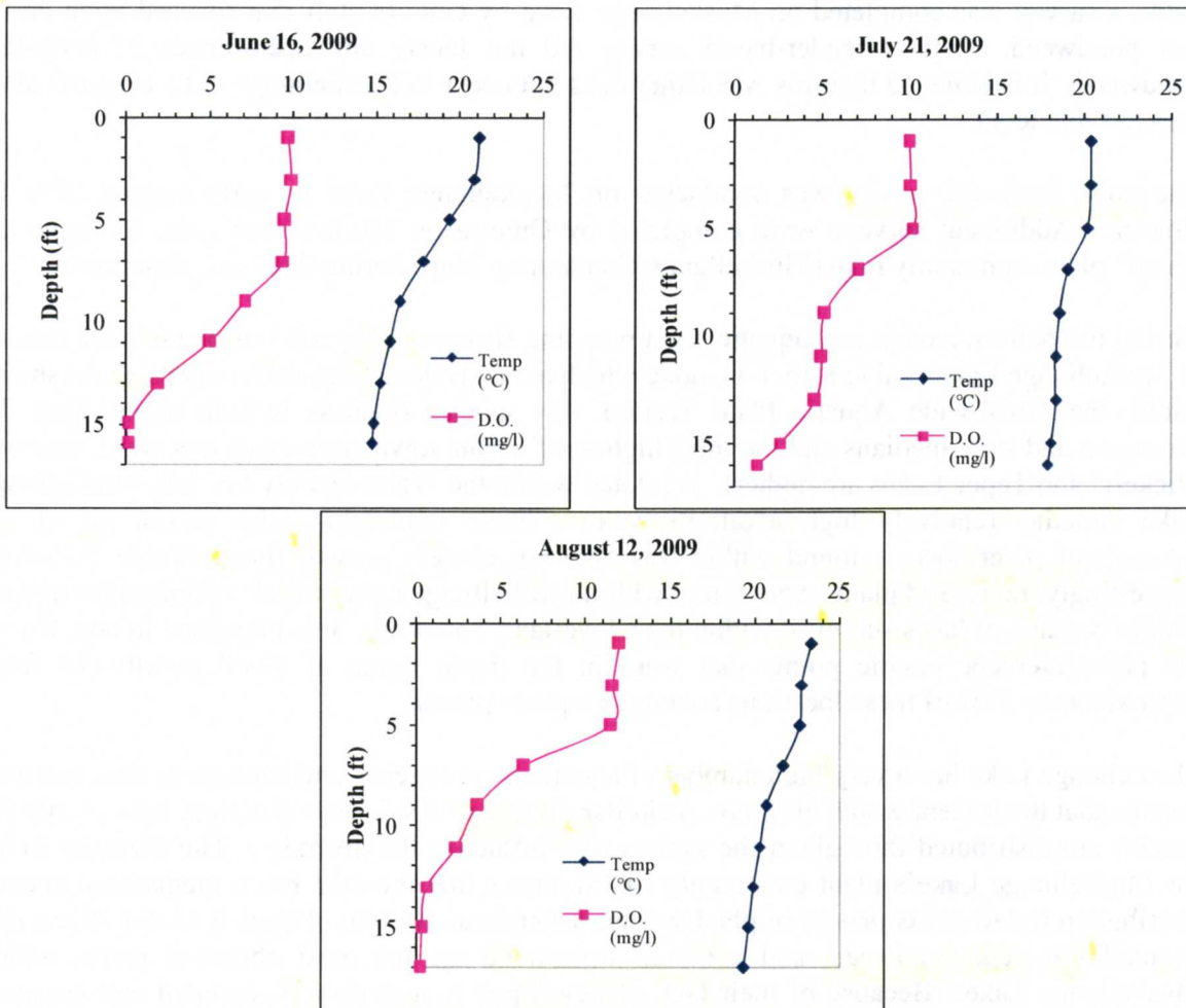
Figure 8.12.3-5. Muskellunge Lake dissolved oxygen and temperature profiles.
