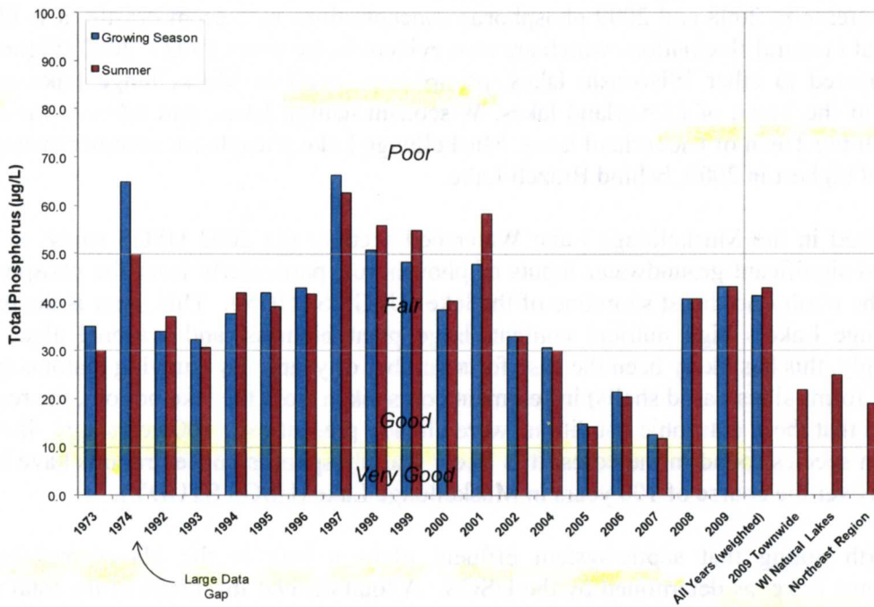
Figure 8.12.3-1. Muskellunge Lake, 2009 town-wide, regional, and state total phosphorus concentrations. Mean values calculated with summer month surface sample data. Water Quality Index values adapted from Lillie and Mason (1983).
